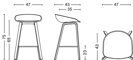
AAS 32 LOW WIDTH 47 CM DEPTH 43 CM HEIGHT 75 CM SEAT HEIGHT 65 CM SEAT DEPTH 35 CM
